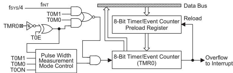
Timer/Event Counter 0
