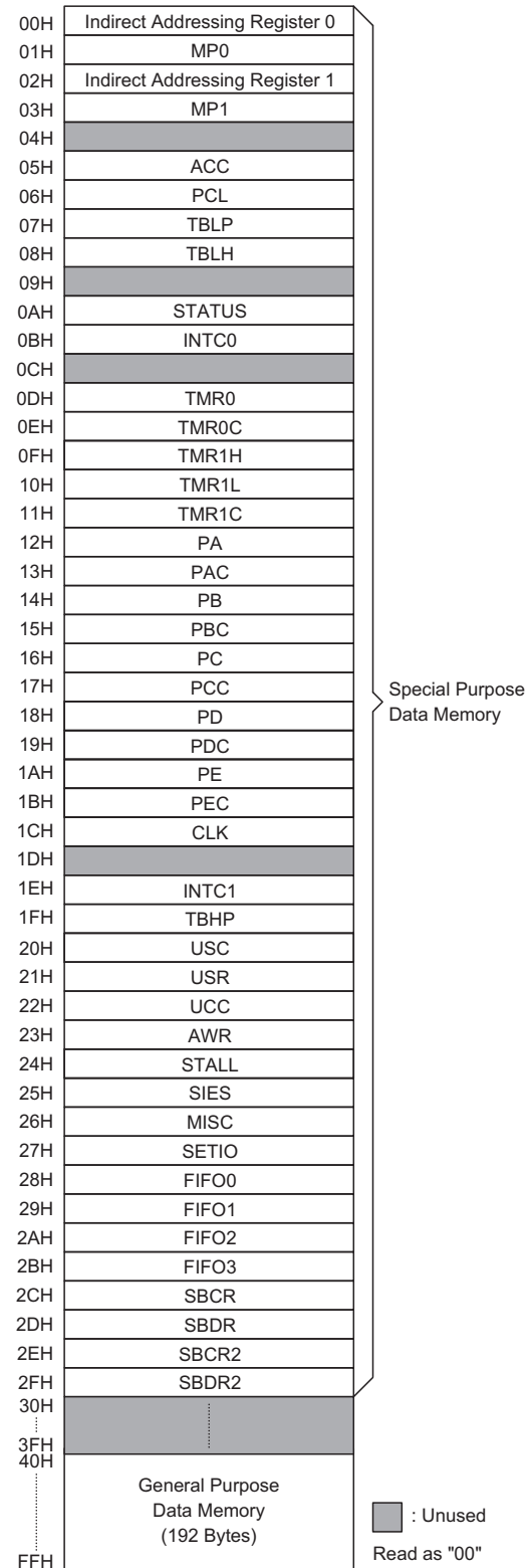
RAM Mapping
