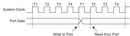
Read/Write Timing
