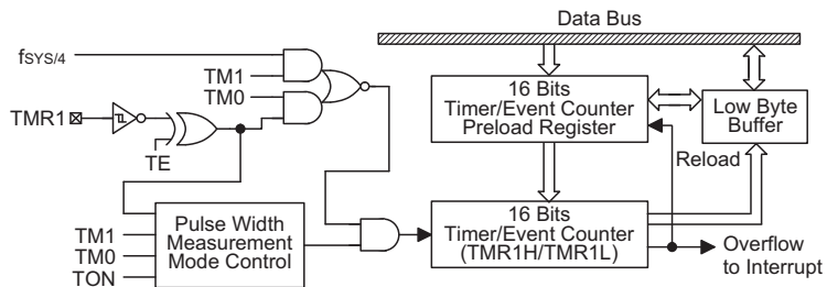
Timer/Event Counter 1
