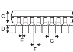
Fig1. Full Lead Packages
