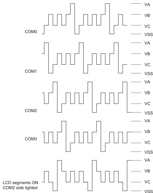
Note: 1/4 duty, 1/3 bias, R type: "VA" VLCD, "VB" 2/3 VLCD, "VC" 1/3 VLCD
