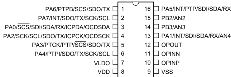
BA45F6730/BA45V6730 16 NSOP-A
