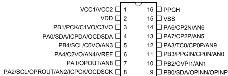
HT45F0059/HT45V0059 16 NSOP-A
