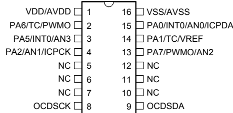
HT66V0021 16 NSOP-A
