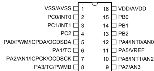
HT66F0041/HT66V0041 16 NSOP-A
