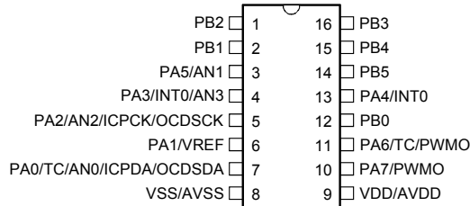
HT66F0031/HT66V0031 16 NSOP-A
