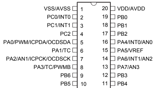
HT66F0041/HT66V0041 20 NSOP-A/SSOP-A
