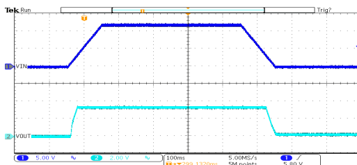
开关响应: HT7133-1 ( V_{IN}=12V , I_{OUT}=0mA , TRISE=TFALL=100ms )
