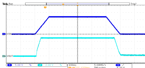
开关响应: HT7150-1 ( V_{IN}=12V , I_{OUT}=0mA , TRISE=TFALL=100ms )
