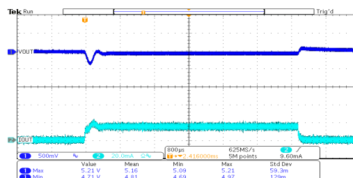
负载瞬态响应: HT7150-1 ( V_{IN}=7V , I_{OUT}=0mA \sim 15mA )
