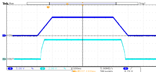
开关响应: HT7150-1 ( V_{IN}=12V , I_{OUT}=30mA , TRISE=TFALL=100ms )
