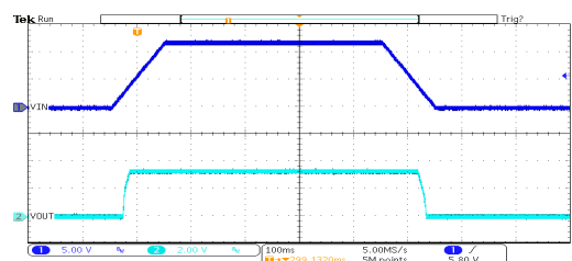
开关响应: HT7133-1 ( V_{IN}=12V , I_{OUT}=30mA , TRISE=TFALL=100ms )
