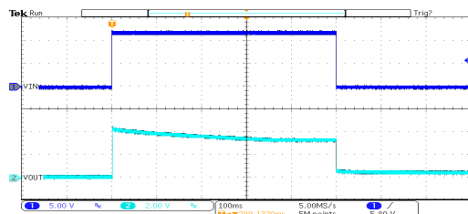
开关响应: HT7133-1 ( V_{IN}=12V , I_{OUT}=0mA , TRISE=TFALL=0.1ms )
