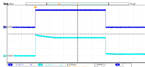
开关响应: HT7150-1 ( V_{IN}=12V , I_{OUT}=0mA , TRISE=TFALL=0.1ms )
