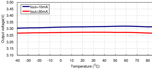
输出电压与温度：HT7133-1 (V IN =V OUT +2V)
