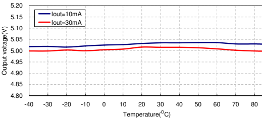
输出电压与温度：HT7150-1 (V IN =V OUT +2V)
