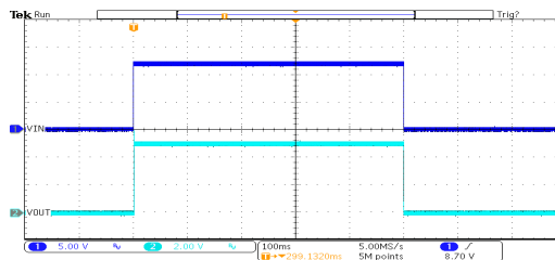
开关响应: HT7150-1 ( V_{IN}=12V , I_{OUT}=30mA , TRISE=TFALL=0.1ms )
