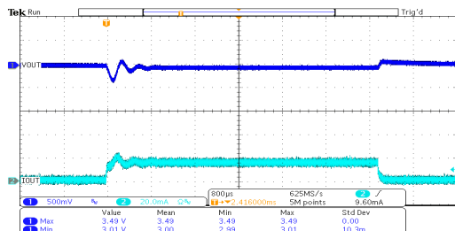
负载瞬态响应: HT7133-1 ( V_{IN}=5.3V , I_{OUT}=0mA \sim 15mA )
