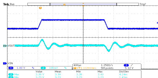
线性瞬态响应: HT7133-1 ( V_{IN}=4.3V \sim 5.3V , I_{OUT}=10mA )
