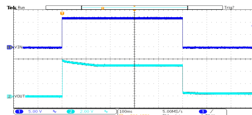
开关响应: HT7150-2 (V IN =12V, I OUT =0mA, TRISE=TFALL=0.1ms)
