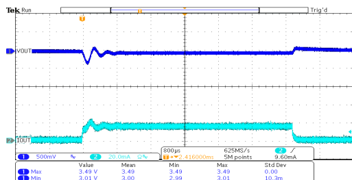
负载瞬态响应: HT7133-2 (V IN =5.3V, I OUT =0mA~15mA)
