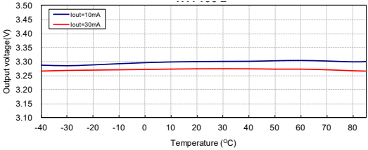
输出电压与温度：HT7133-2 (V IN =V OUT +2V)
