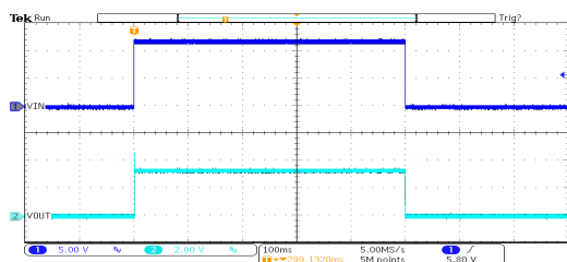
开关响应: HT7133-2 ( V_{IN}=12V , I_{OUT}=30mA , TRISE=TFALL=0.1ms )
