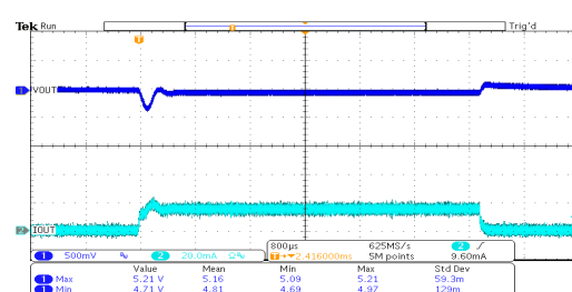
负载瞬态响应: HT7150-2 (V IN =7V, I OUT =0mA~15mA)
