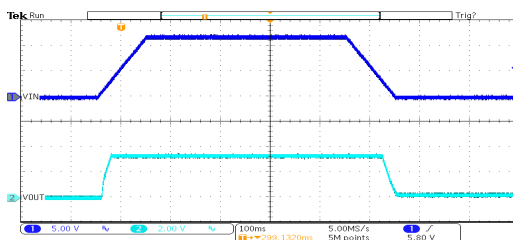
开关响应: HT7133-2 (V IN =12V, I OUT =0mA, TRISE=TFALL=100ms)
