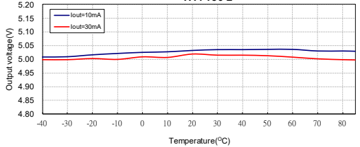
输出电压与温度：HT7150-2 (V IN =V OUT +2V)
