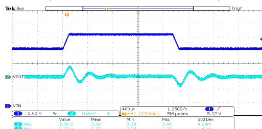
线性瞬态响应: HT7133-2 (V IN =4.3V~5.3V, I OUT =10mA)
