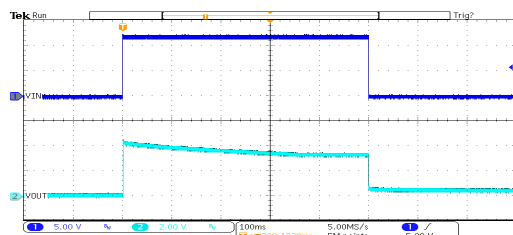
开关响应: HT7133-2 (V IN =12V, I OUT =0mA, TRISE=TFALL=0.1ms)
