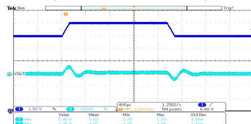
线性瞬态响应: HT7150-2 (V IN =6V~7V, I OUT =10mA)
