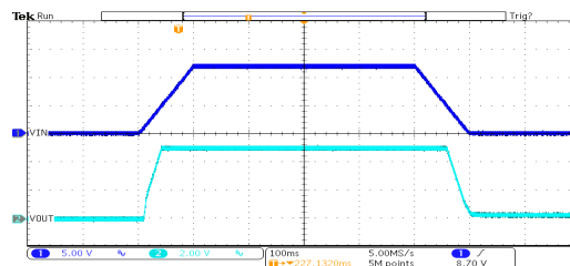
开关响应: HT7150-2 (V IN =12V, I OUT =0mA, TRISE=TFALL=100ms)
