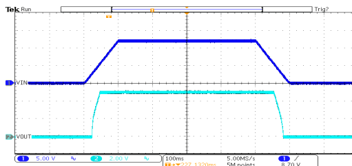
开关响应: HT7150-3 ( V_{IN}=12V , I_{OUT}=30mA , TRISE=TFALL=100ms )
