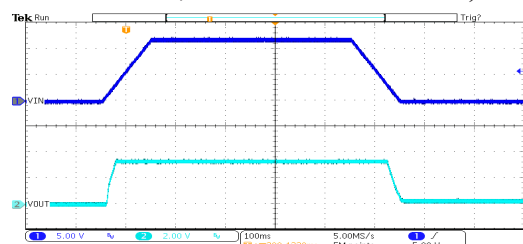
开关响应: HT7133-3 ( V_{IN}=12V , I_{OUT}=0mA , TRISE=TFALL=100ms )
