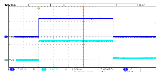
开关响应: HT7150-3 ( V_{IN}=12V , I_{OUT}=0mA , TRISE=TFALL=0.1ms )
