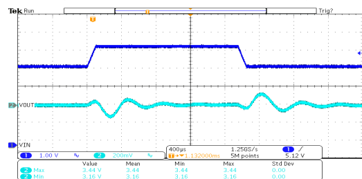
线性瞬态响应: HT7133-3 ( V_{IN}=4.3V \sim 5.3V , I_{OUT}=10mA )
