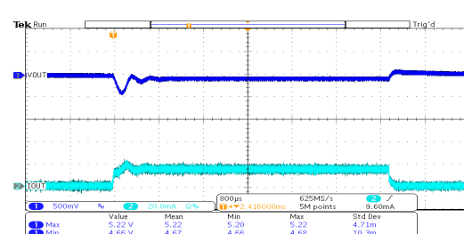
负载瞬态响应: HT7150-3 ( V_{IN}=7V , I_{OUT}=0mA to 15mA )
