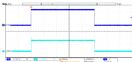
开关响应: HT7133-3 ( V_{IN}=12V , I_{OUT}=30mA , TRISE=TFALL=0.1ms )
