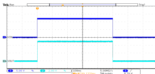
开关响应: HT7150-3 ( V_{IN}=12V , I_{OUT}=30mA , TRISE=TFALL=0.1ms )
