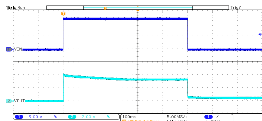
开关响应: HT7133-3 ( V_{IN}=12V , I_{OUT}=0mA , TRISE=TFALL=0.1ms )
