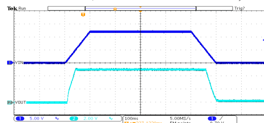
开关响应: HT7150-3 ( V_{IN}=12V , I_{OUT}=0mA , TRISE=TFALL=100ms )
