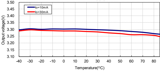
输出电压与温度：HT7133-3 (V IN =V OUT +2V)
