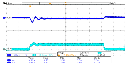
负载瞬态响应: HT7133-3 ( V_{IN}=5.3V , I_{OUT}=0mA to 15mA )
