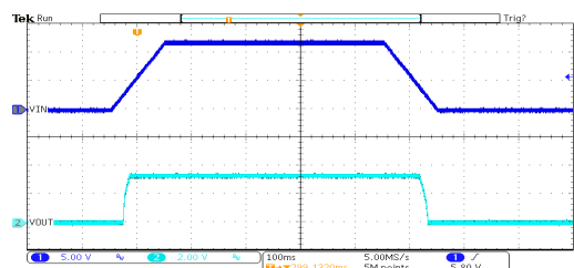
开关响应: HT7133-3 ( V_{IN}=12V , I_{OUT}=30mA , TRISE=TFALL=100ms )
