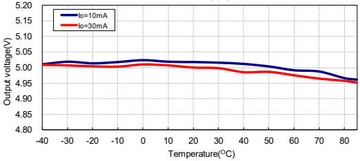
输出电压与温度：HT7150-3 (V IN =V OUT +2V)
