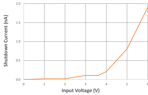
关机电流 vs. 输入电压
