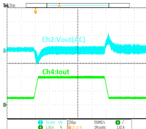
负载瞬态 ( I_{OUT}=0.5A \leftrightarrow 2A , C_{FB}=47pF )
