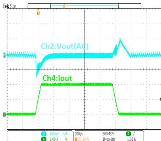
负载瞬态 ( I_{OUT}=1mA \leftrightarrow 2A , C_{FB}=47pF )
