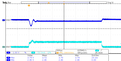
负载瞬态响应：HT7533-1 ( V_{IN} = 5.3V , I_{OUT} = 0mA \sim 40mA )
