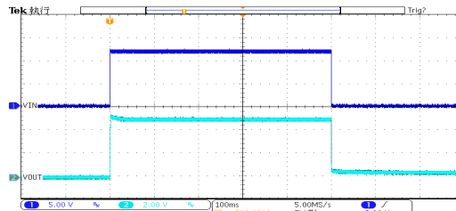
开关响应: HT7550-1 ( V_{IN}=12V , I_{OUT}=0mA , TRISE=TFALL=0.1ms )
