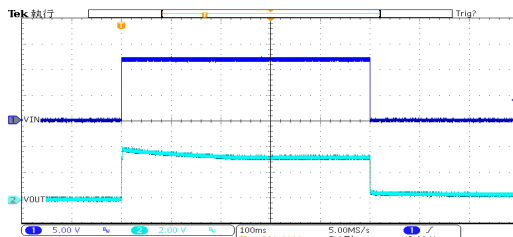
开关响应: HT7533-1 ( V_{IN}=12V , I_{OUT}=0mA , TRISE=TFALL=0.1ms )
