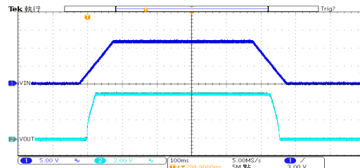
开关响应: HT7550-1 ( V_{IN}=12V , I_{OUT}=100mA , TRISE=TFALL=100ms )
