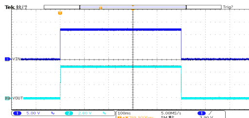
开关响应: HT7550-1 ( V_{IN}=12V , I_{OUT}=100mA , TRISE=TFALL=0.1ms )
