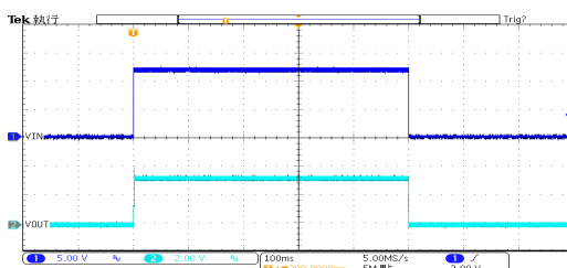
开关响应: HT7533-1 ( V_{IN}=12V , I_{OUT}=100mA , TRISE=TFALL=0.1ms )
