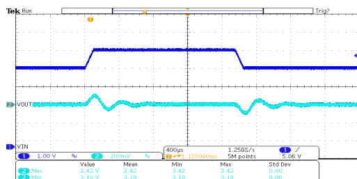
线性瞬态响应: HT7533-1 ( V_{IN}=4.3V\sim5.3V , I_{OUT}=10mA )
