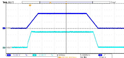
开关响应: HT7550-3 ( V_{IN}=12V , I_{OUT}=100mA , TRISE=TFALL=0.1ms )
