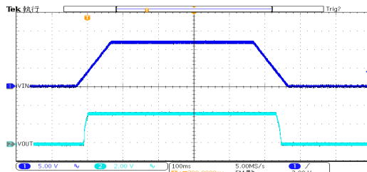
开关响应: HT7533-3 ( V_{IN}=12V , I_{OUT}=100mA , TRISE=TFALL=100ms )
