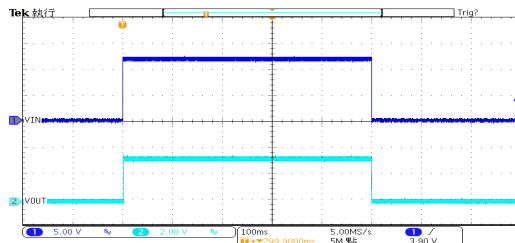
开关响应: HT7533-3 ( V_{IN}=12V , I_{OUT}=100mA , TRISE=TFALL=0.1ms )
