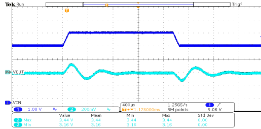
线性瞬态响应: HT7533-3 ( V_{IN}=4.3V\sim5.3V , I_{OUT}=10mA )
