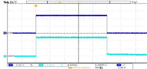
开关响应: HT7550-3 ( V_{IN}=12V , I_{OUT}=0mA , TRISE=TFALL=100ms )
