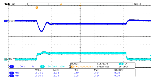
负载瞬态响应：HT7533-3 ( V_{IN} = 5.3V , I_{OUT} = 0mA \sim 40mA )
