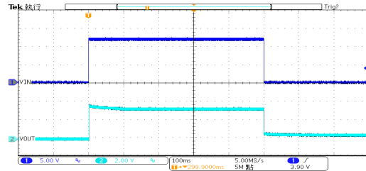
开关响应: HT7533-3 ( V_{IN}=12V , I_{OUT}=0mA , TRISE=TFALL=100ms )
